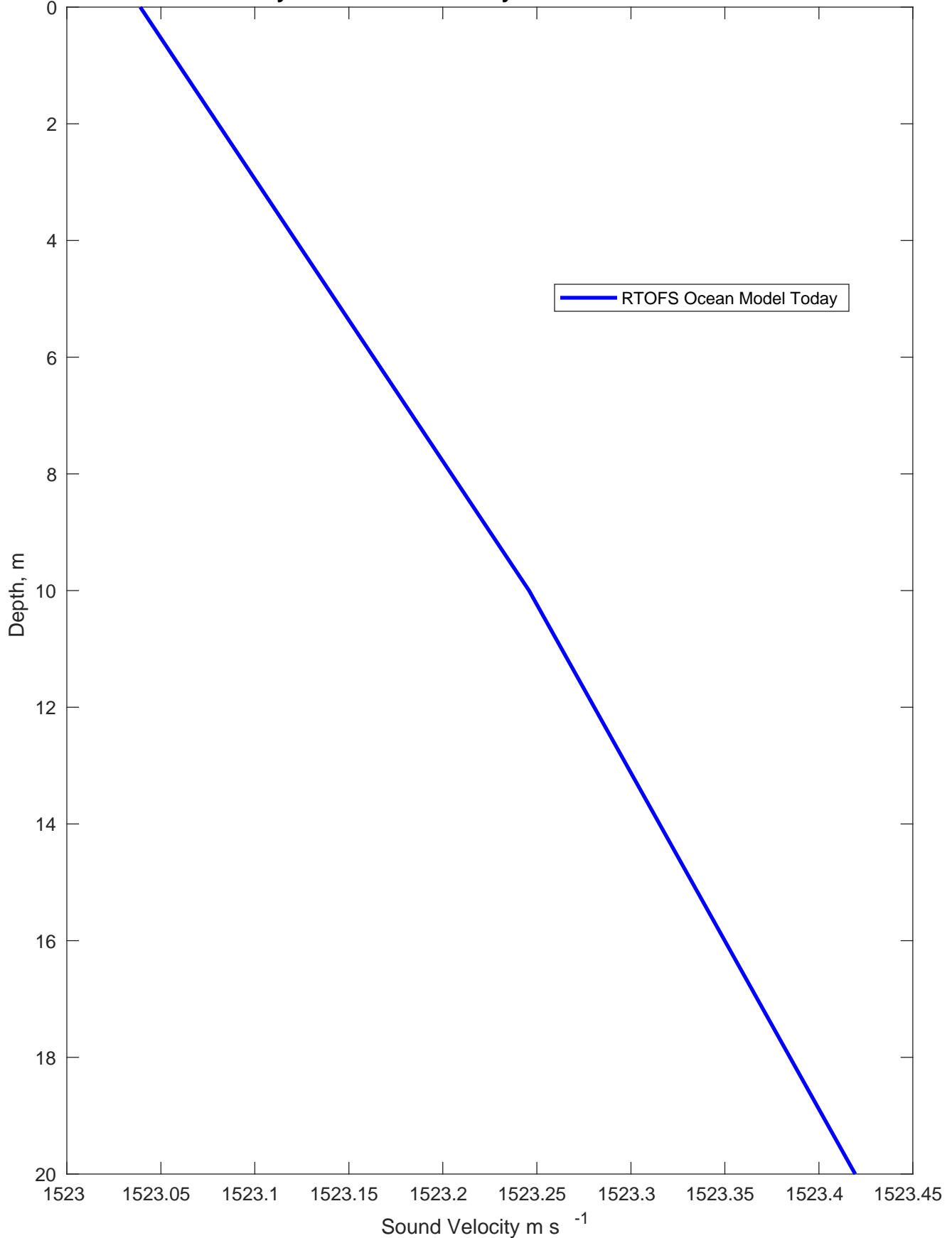
Sound Velocity Profile for TABS Buoy F on 08-Dec-2020 00:00:00
